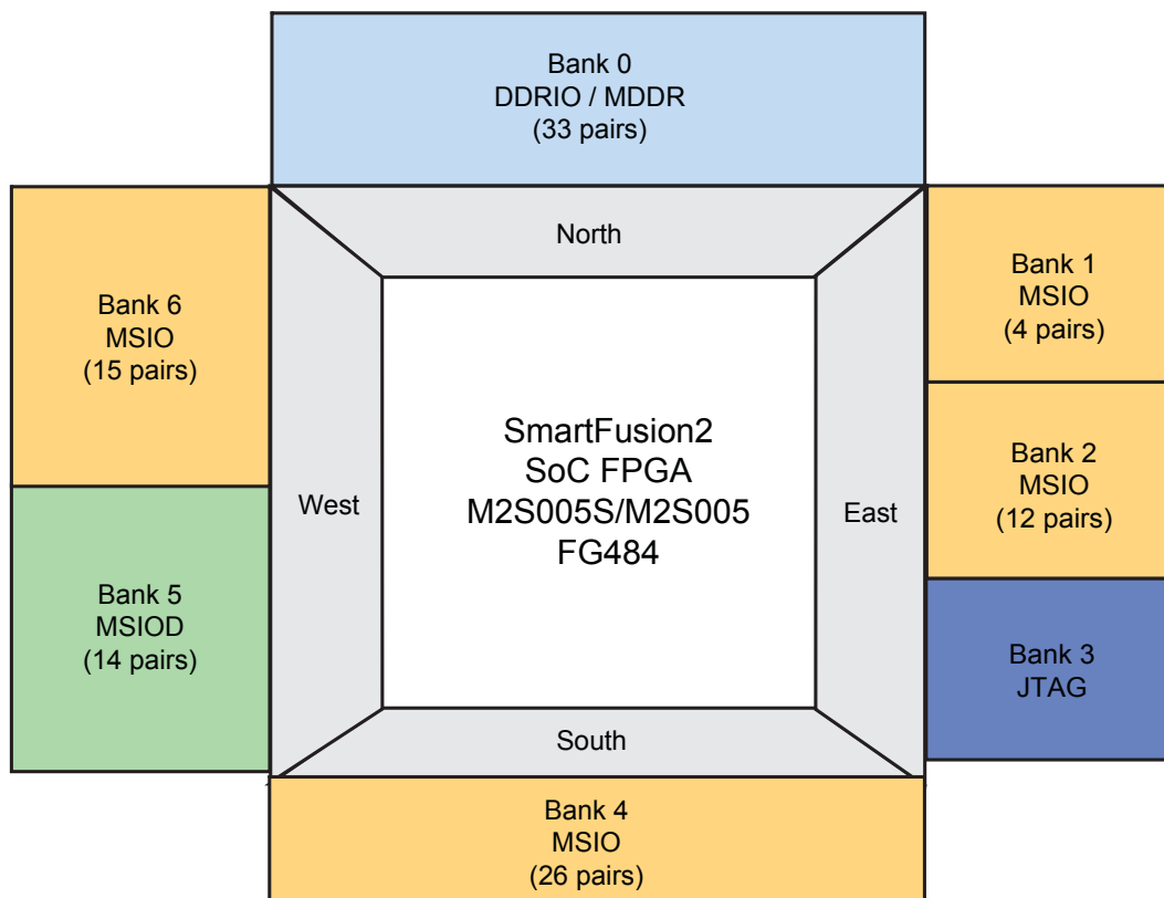
Figure 11 • SmartFusion2 M2S005S/M2S005-FG484 I/O Bank Locations
