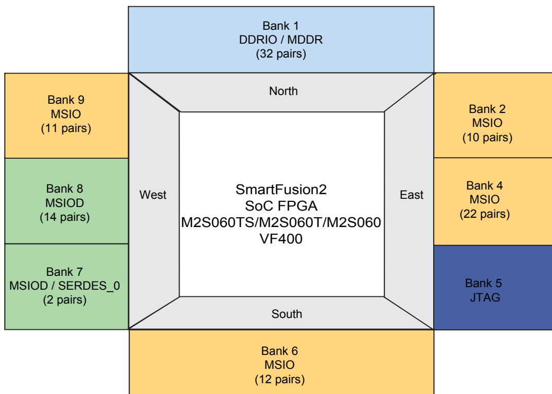
Figure 13 • SmartFusion2 M2S060TS/M2S060T/M2S060-VF400 I/O Bank Locations
