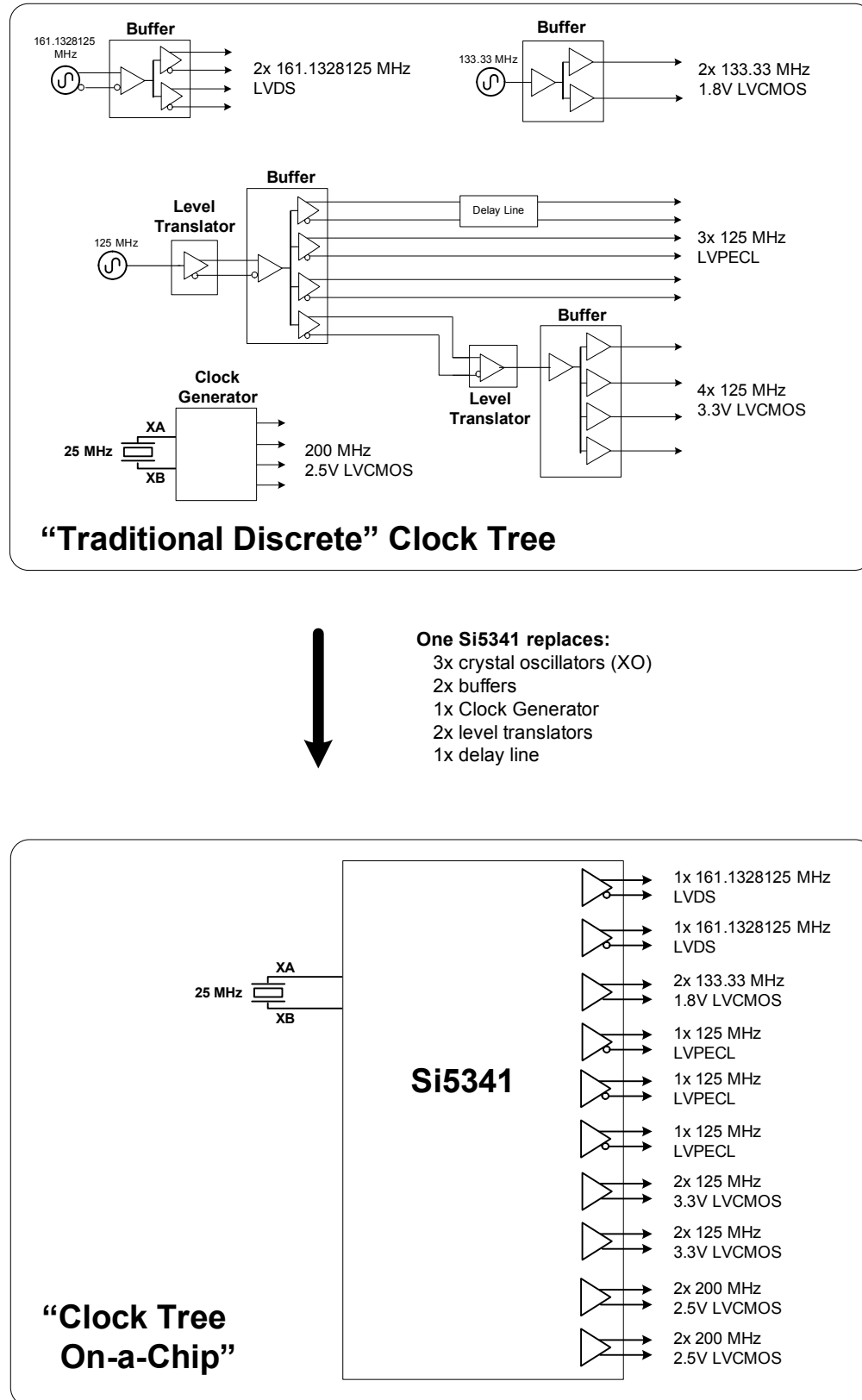
Figure 6.1. Using the Si5341 to Replace a Traditional Clock Tree
