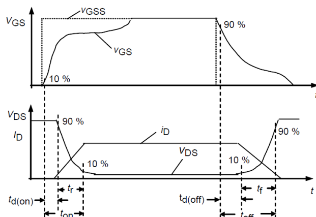
Figure 32. Resistive Switching Time Description
