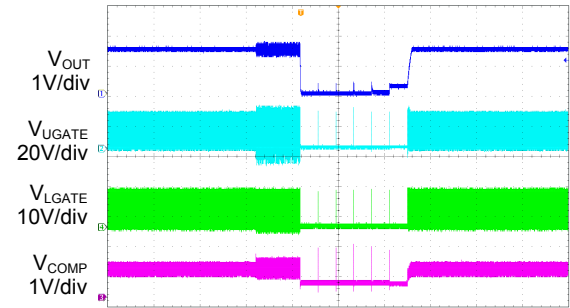
Under Voltage Protection ( V_{IN} = 12V , V_{OUT} = 1.5V )
