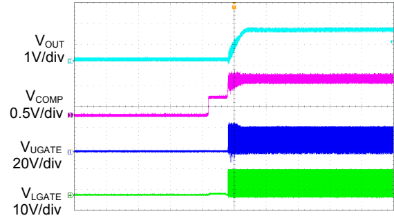
Enable-on Waveform ( V_{IN} = 12V , V_{OUT} = 1.5V , I_{OUT} = 0A )
