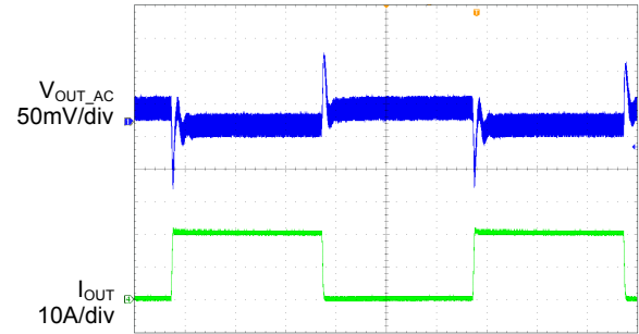
Load Transient Response ( V_{IN} = 12V , V_{OUT} = 1.5V , I_{OUT} = 0A to 20A )
