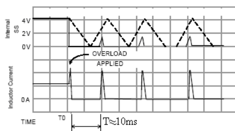
Figure 4. Hiccuped Over Current Protection
