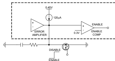
Figure 1. Chip Enable Function
