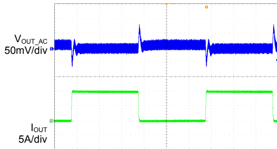
Load Transient Response ( V_{IN} = 12V , V_{OUT} = 1.5V , I_{OUT} = 0A to 10A )
