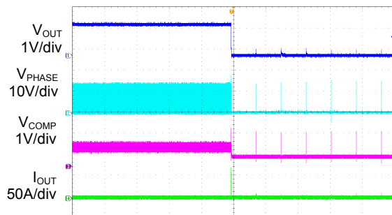
Over Current Protection ( V_{IN} = 12V , V_{OUT} = 1.5V )
