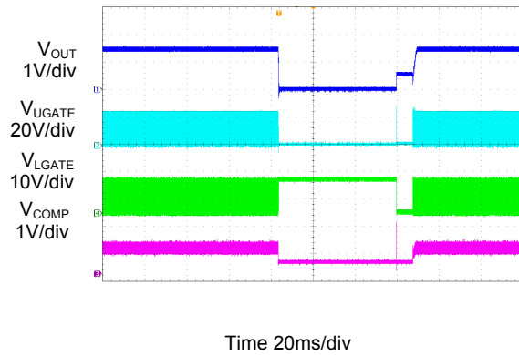
Over Voltage Protection ( V_{IN} = 12V , V_{OUT} = 1.5V )
