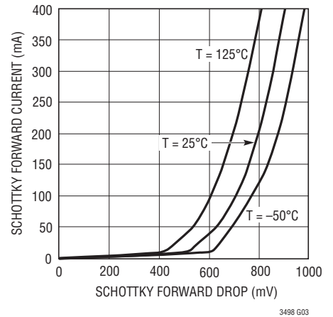
LED Schottky Forward Voltage Drop
