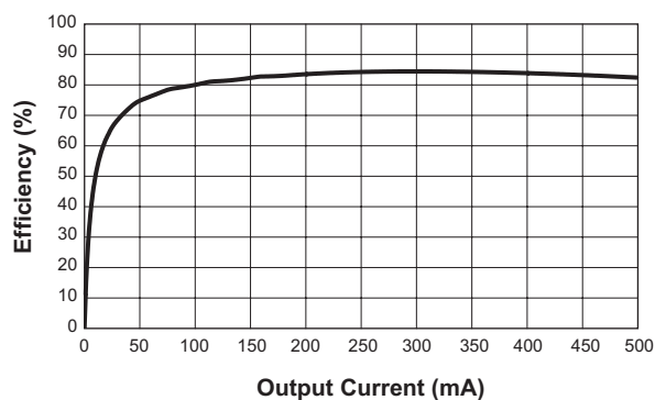
Main Boost Efficiency (V OUT = 12V)
