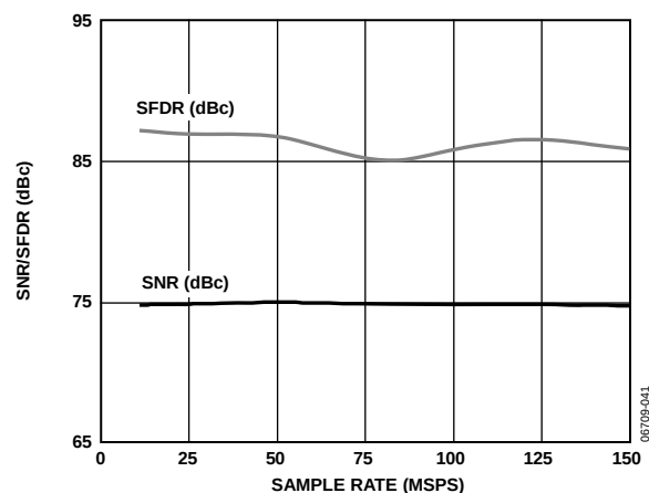
Figure 42. AD6655-150 Single-Tone SNR/SFDR vs. Sample Rate ( f_s ) with f_{IN} = 2.3 MHz
