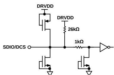
Figure 14. Equivalent SDIO/DCS Circuit or SMI SDFS Circuit
