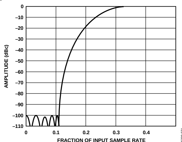
Figure 73. Half-Band Filter High-Pass Response
