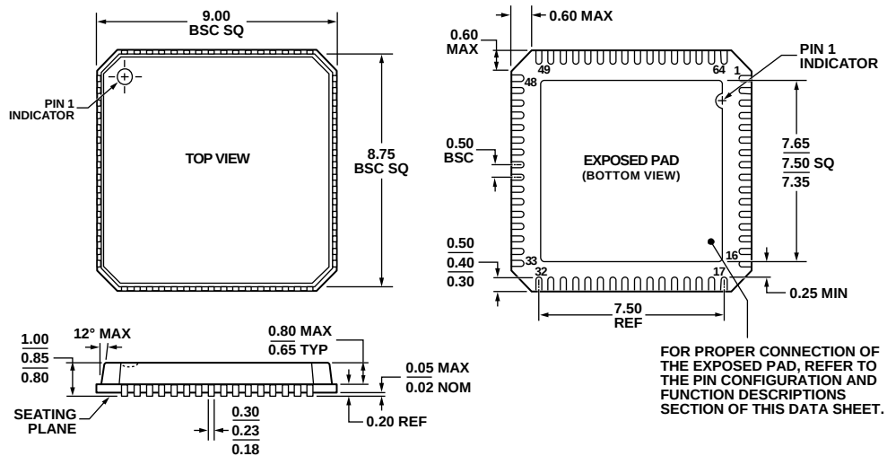
Figure 104. 64-Lead Lead Frame Chip Scale Package [LFCSP_VQ] 9 mm × 9 mm Body, Very Thin Quad (CP-64-6) Dimensions shown in millimeters
