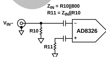
Figure 6. Single-Ended Input Impedance
