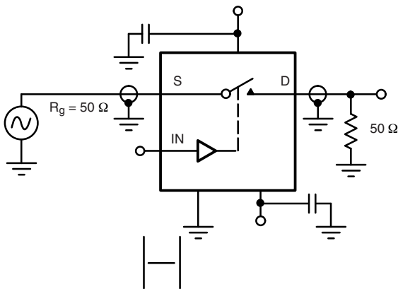
Figure 3. Off Isolation
