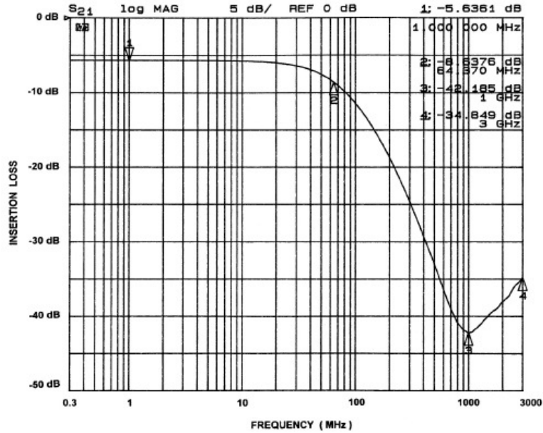
Figure 1. Insertion Loss vs. Frequency (A2-C2 to GND B2)
