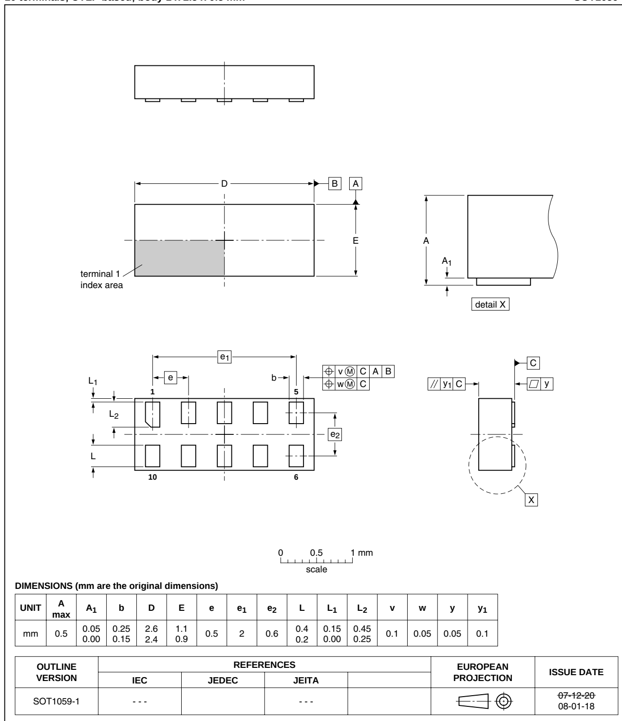
Fig 12. Package outline SOT1059-1 (XSON10U)
