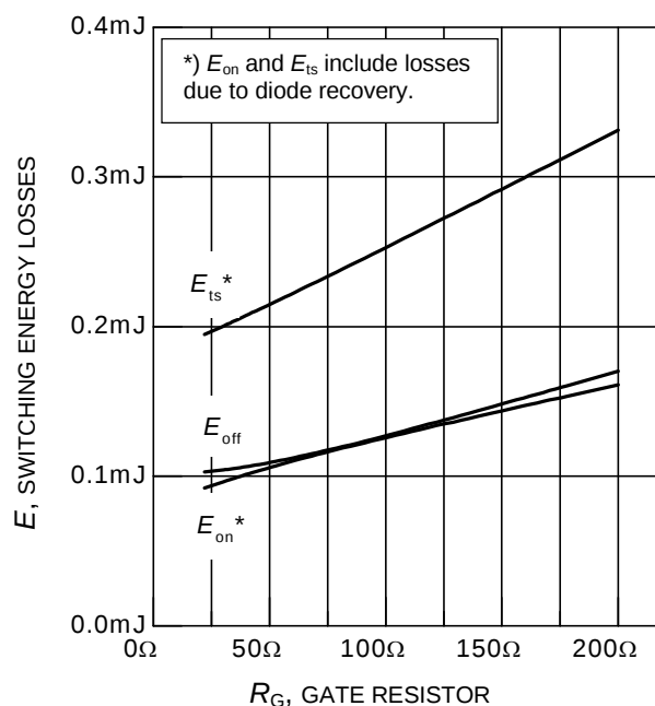
Figure 14. Typical switching energy losses as a function of gate resistor (inductive load, T_j = 150^\circ\text{C} , V_{CE} = 400\text{V} , V_{GE} = 0/+15\text{V} , I_C = 4\text{A} , Dynamic test circuit in Figure E)
