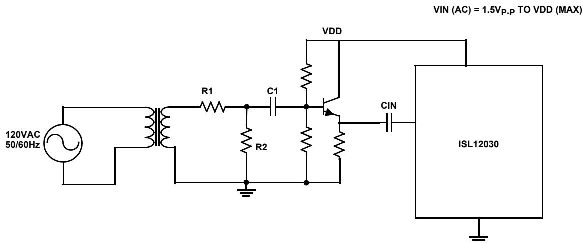
FIGURE 9. USING THE V_{DD} SUPPLY TO GATE THE AC INPUT
