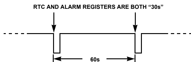
FIGURE 2. \overline{\text{IRQ}} WAVEFORM
