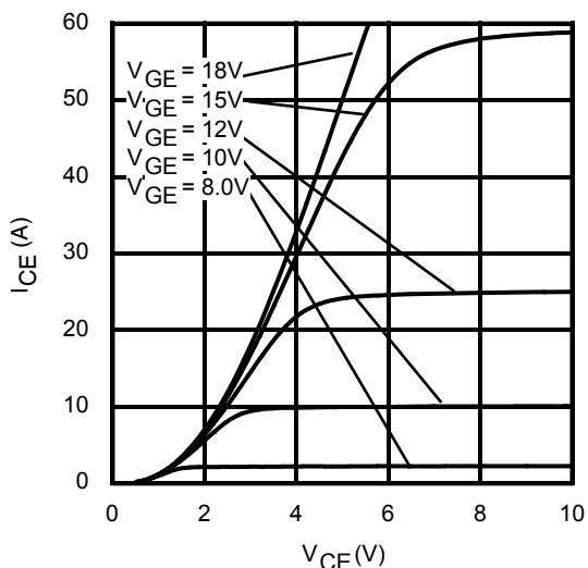
Fig. 8 - Typ. IGBT Output Characteristics T J = 150°C; t p = 20μs
