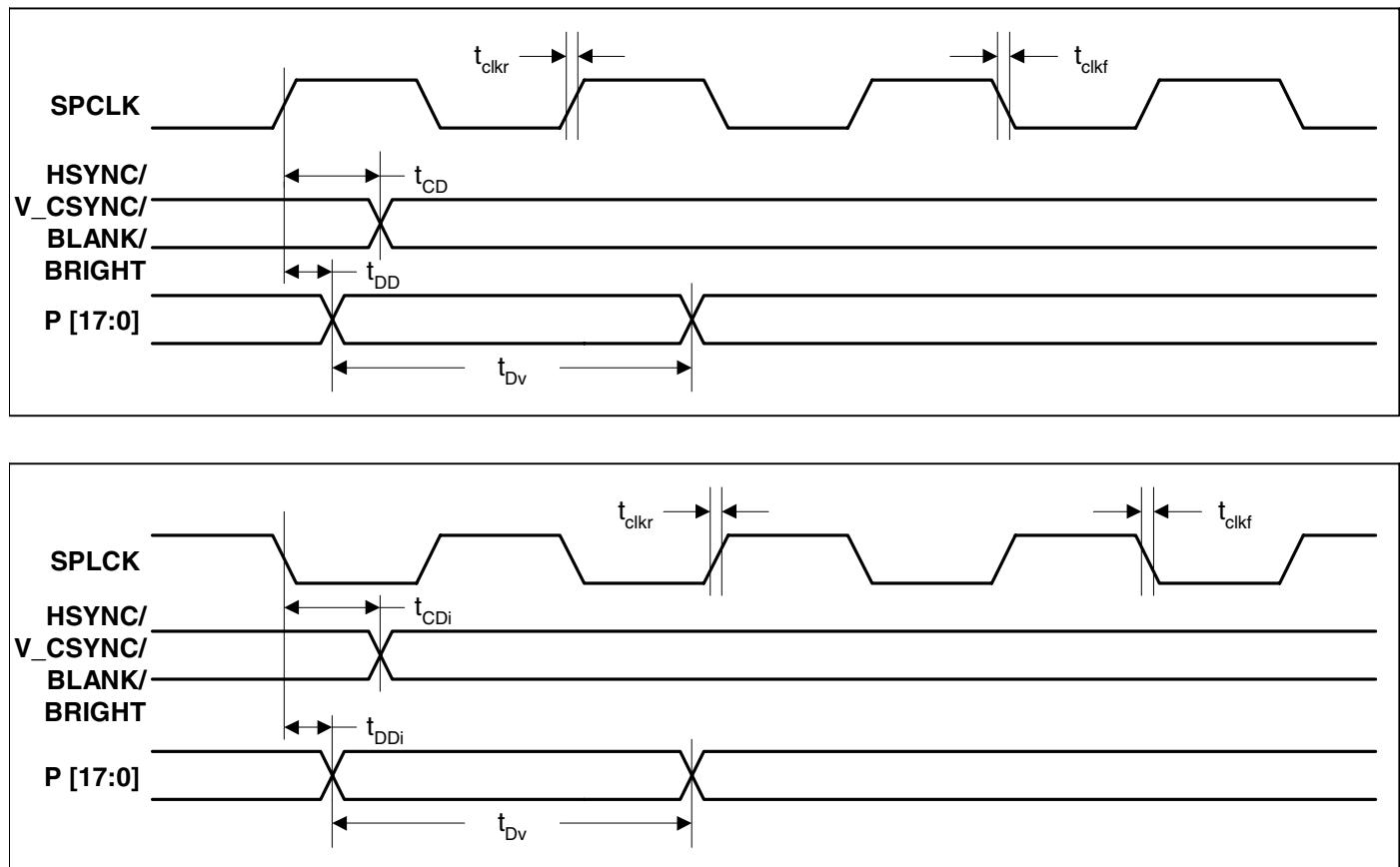
Figure 22. LCD Timing Measurement
