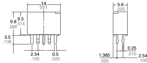
Self-clinching terminal
