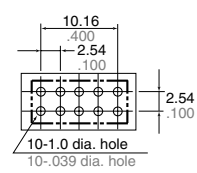
PC board pattern (Copper-side view)
