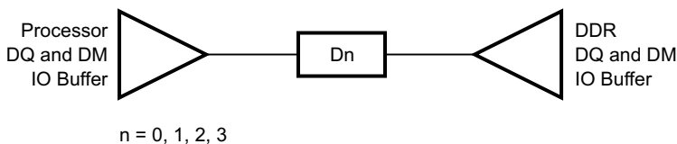
Figure 8-75. DQ/DM Topology
