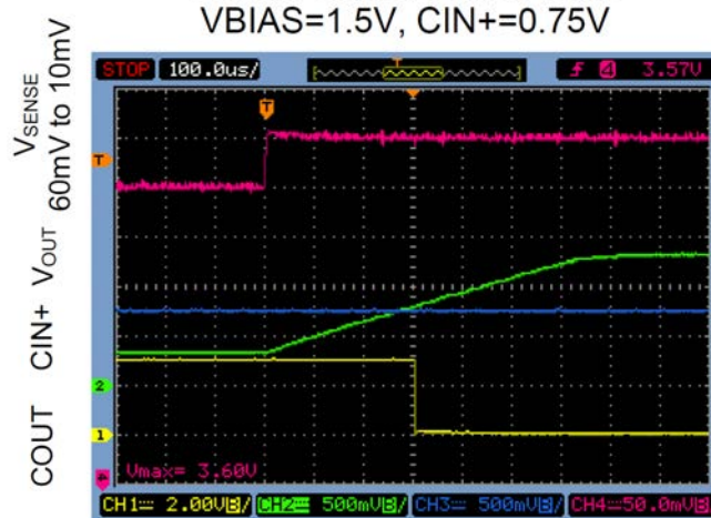
Current Limiter Falling Edge VBIAS=1.5V, CIN+=0.75V
