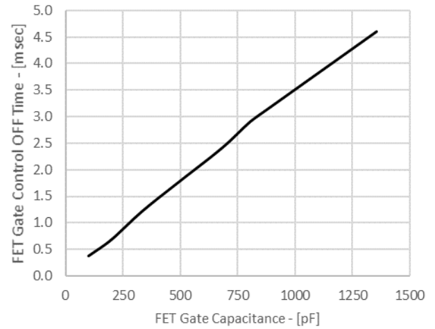
FET OFF Time vs Gate Capacitance
