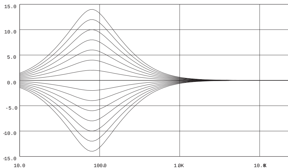
Figure 4. Bass Control @ f_C = 80\text{Hz} , Q = 1
