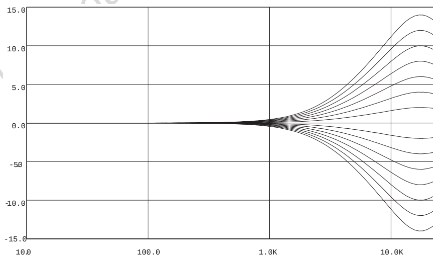
Figure 11. Treble Control @ f_C = 17.5\text{kHz}
