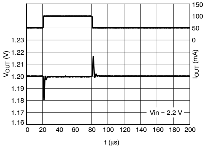
Figure 31. Load Transient Response Load Step 50 mA to 100 mA NCP4688xx12
