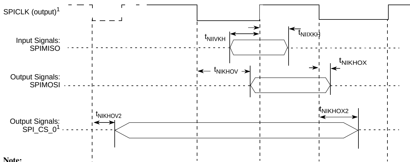
Figure 9. SPI AC timing in master mode (internal clock) diagram
