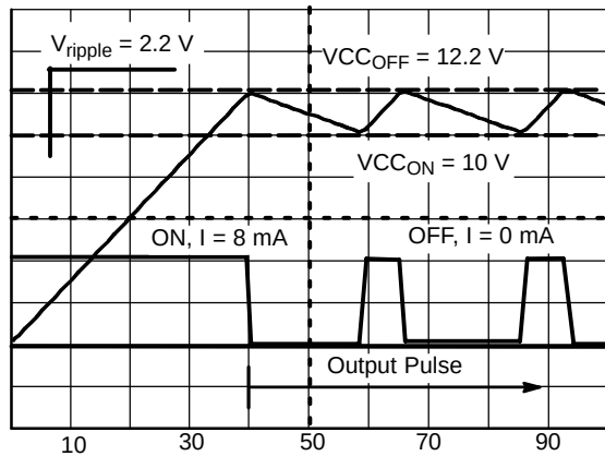
Figure 18. The Charge/Discharge Cycle Over a 10\text{ }\mu\text{F} V_{CC} Capacitor
