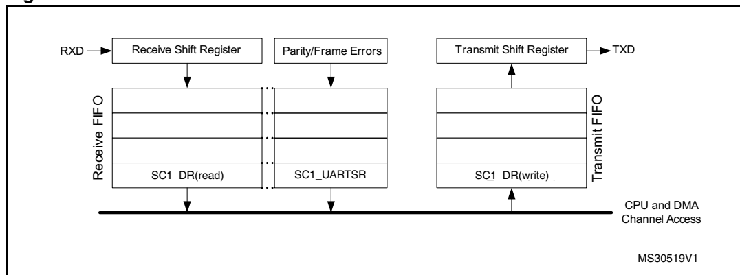
Figure 11. UART FIFOs
