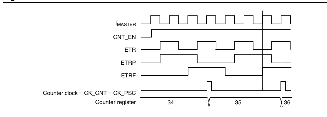
Figure 28. Control circuit in external clock mode 2
