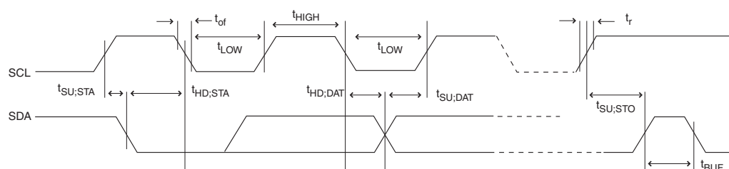
Figure 27-1. 2-wire Serial Bus Timing
