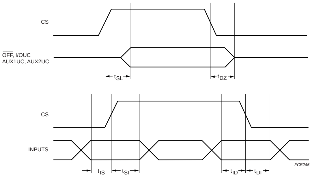
Fig.7 Chip select.
