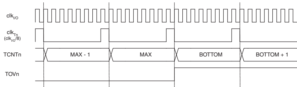
Figure 13-9. Timer/Counter Timing Diagram, with Prescaler ( f_{\text{clk}_{I/O}}/8 )
