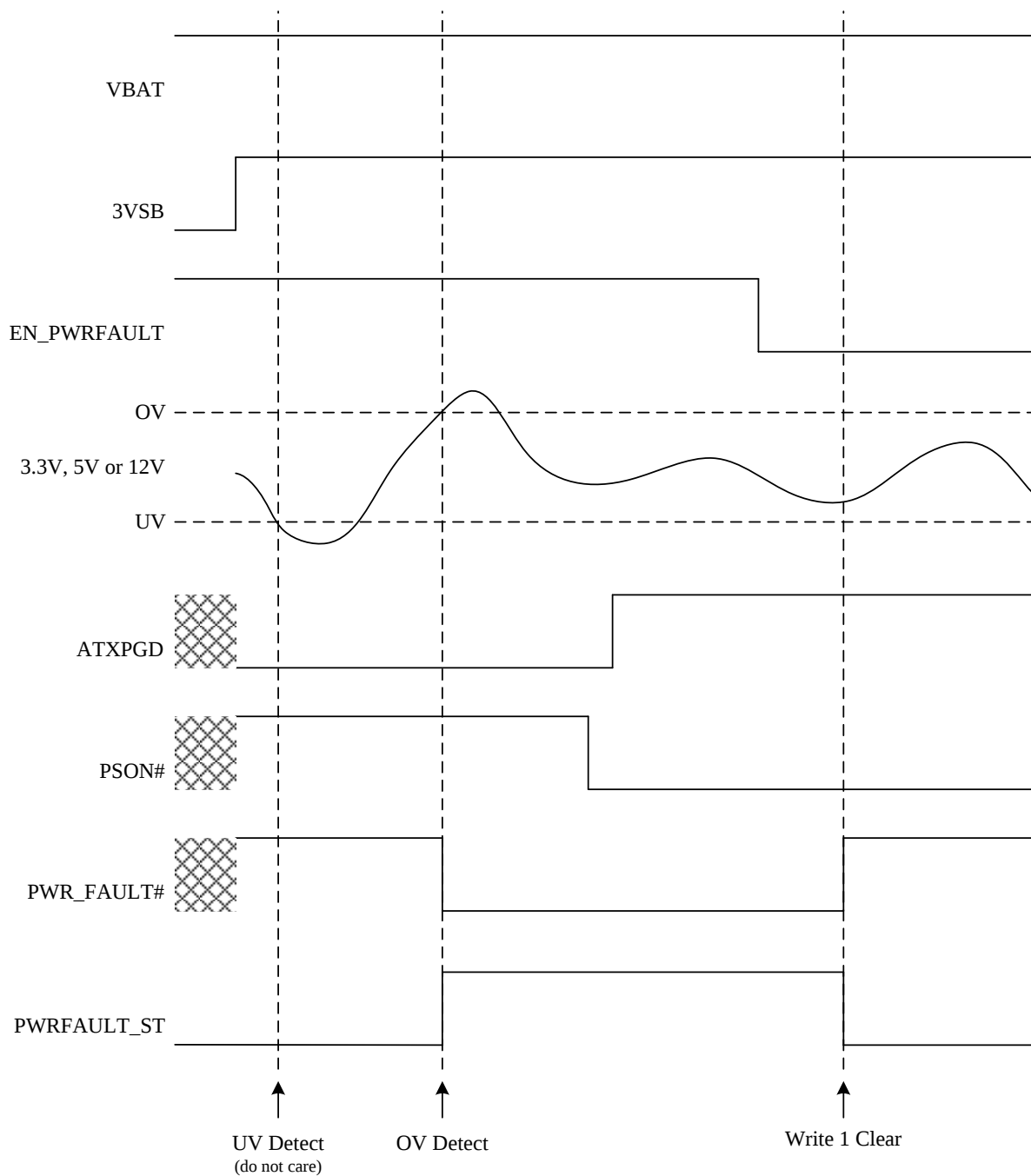
Figure 5-12 Power Fault (EN_PWRFAULT=1, ATXPGD=0, OV Detect)
