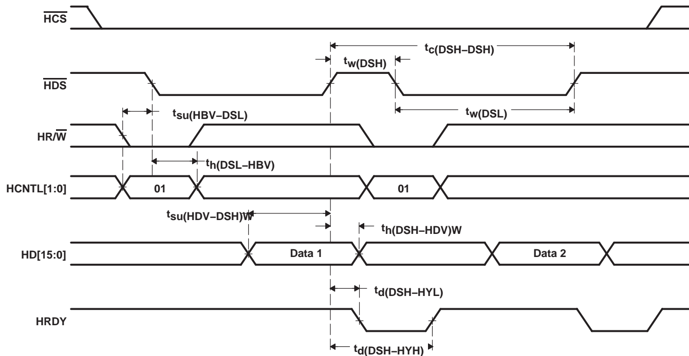
Figure 5-30. Multiplexed Write Timings With \overline{H_{AS}} Held High
