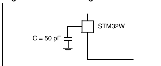
Figure 51. Pin loading conditions
