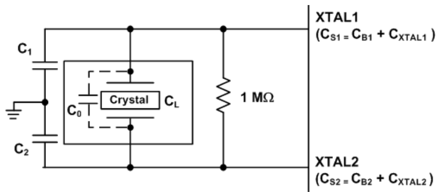
Figure 9.1 Typical Crystal Circuit
