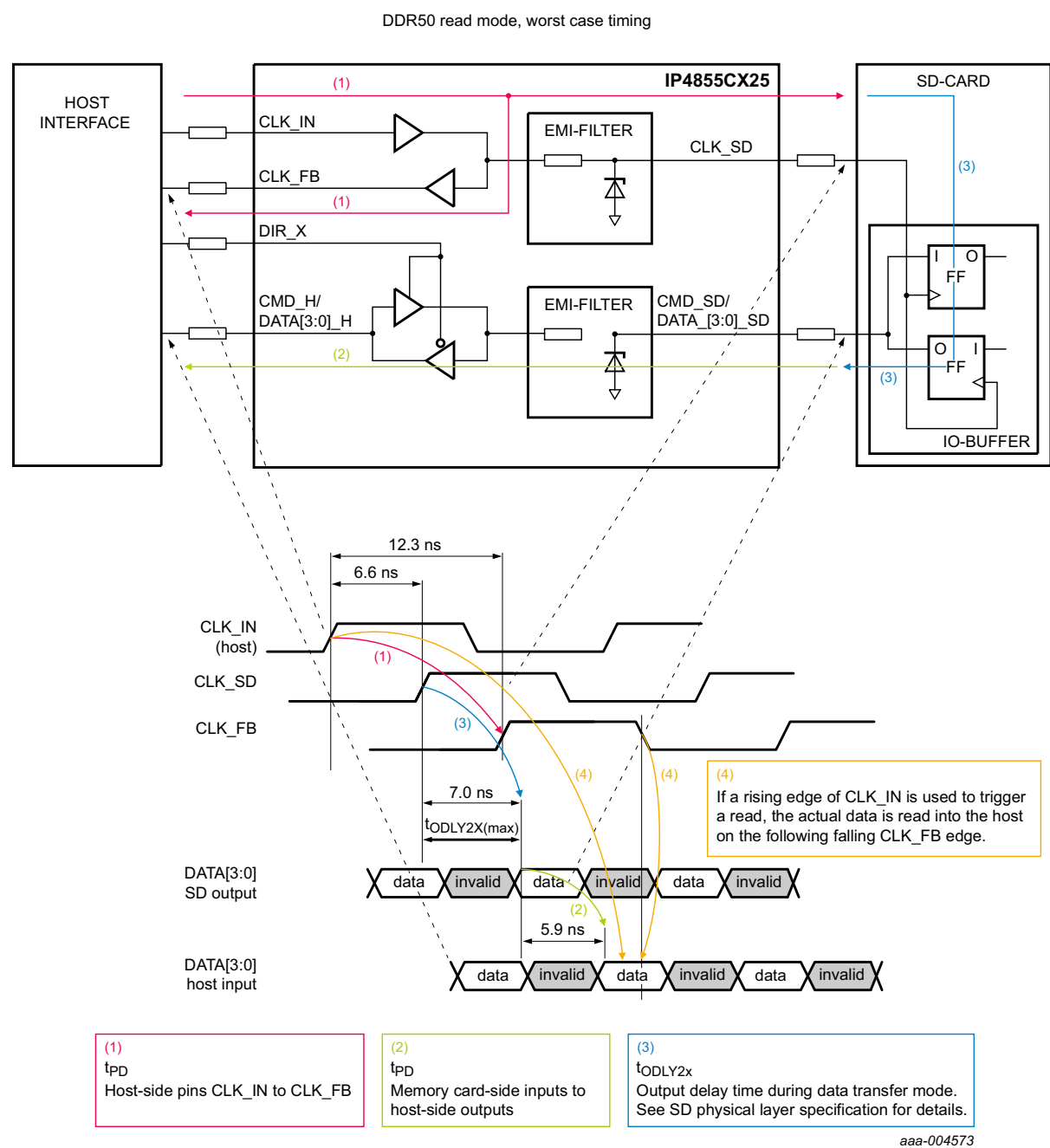
Fig 12. Detailed description of a DDR50 read cycle, worst case timing
