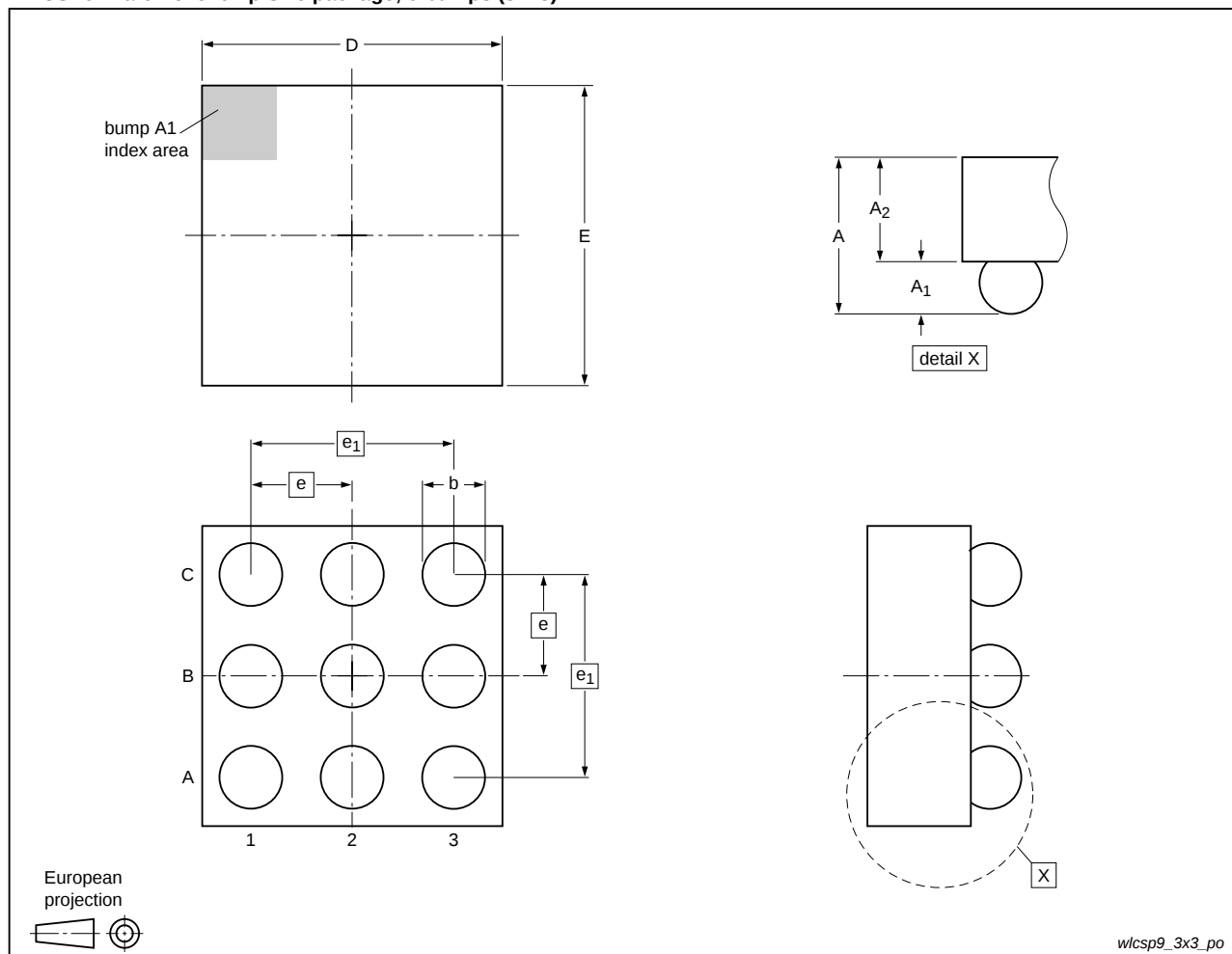
Fig 7. Package outline WLCSP9 (IP4309CX9)
