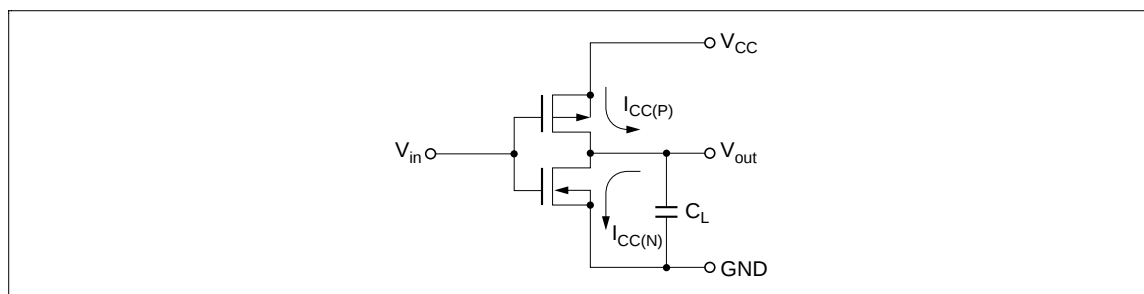
Figure 6 Inverter circuit
