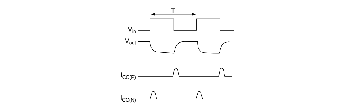
Figure 7 Operating Voltage and current of inverter circuit
