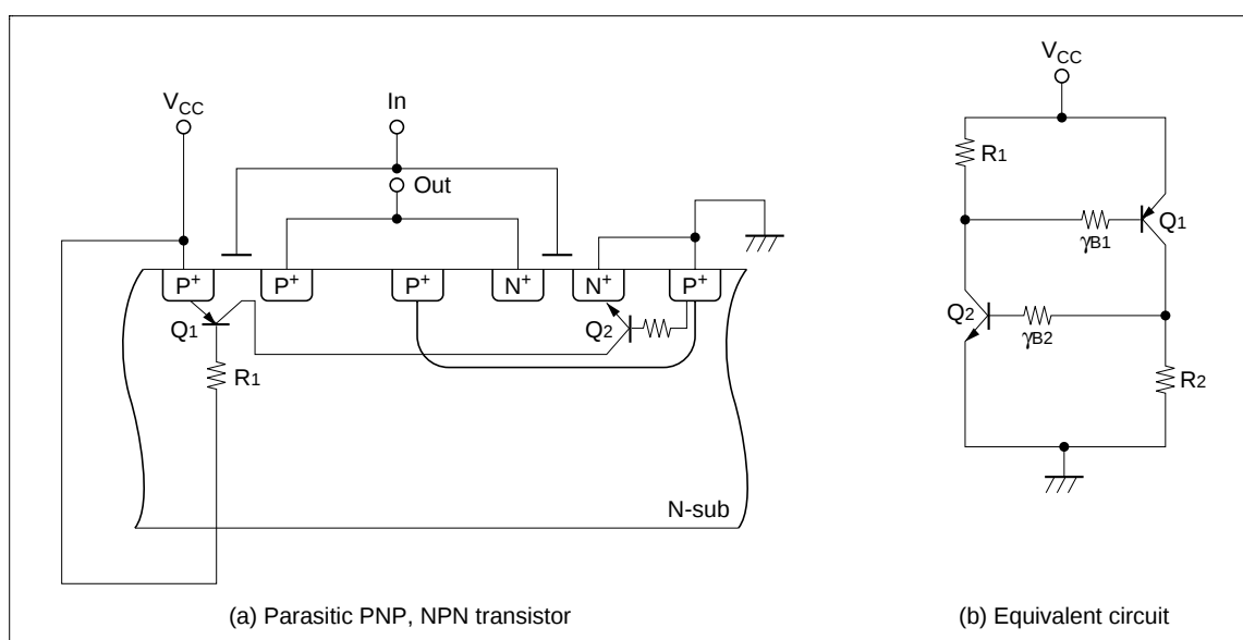
Figure 4 Parasitic Thyristor
