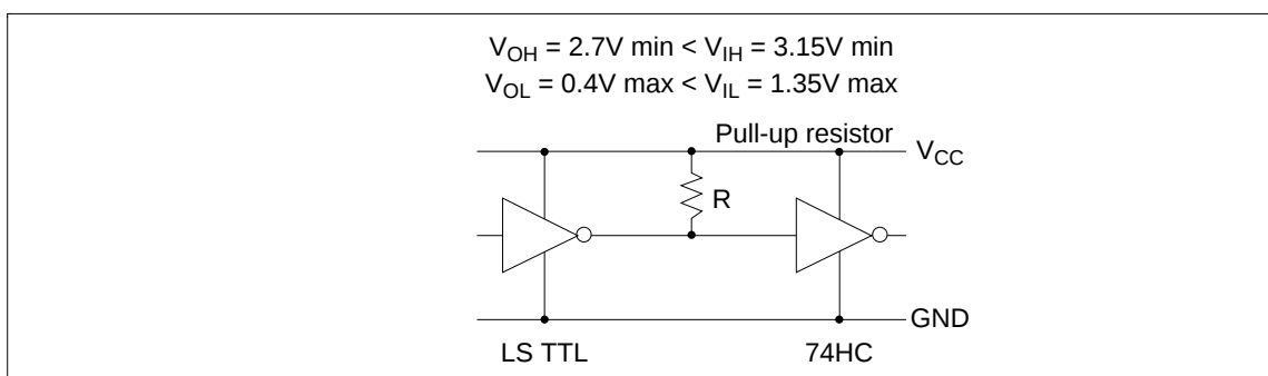
Figure 25 Interfacing LS-TTL to 74HC
