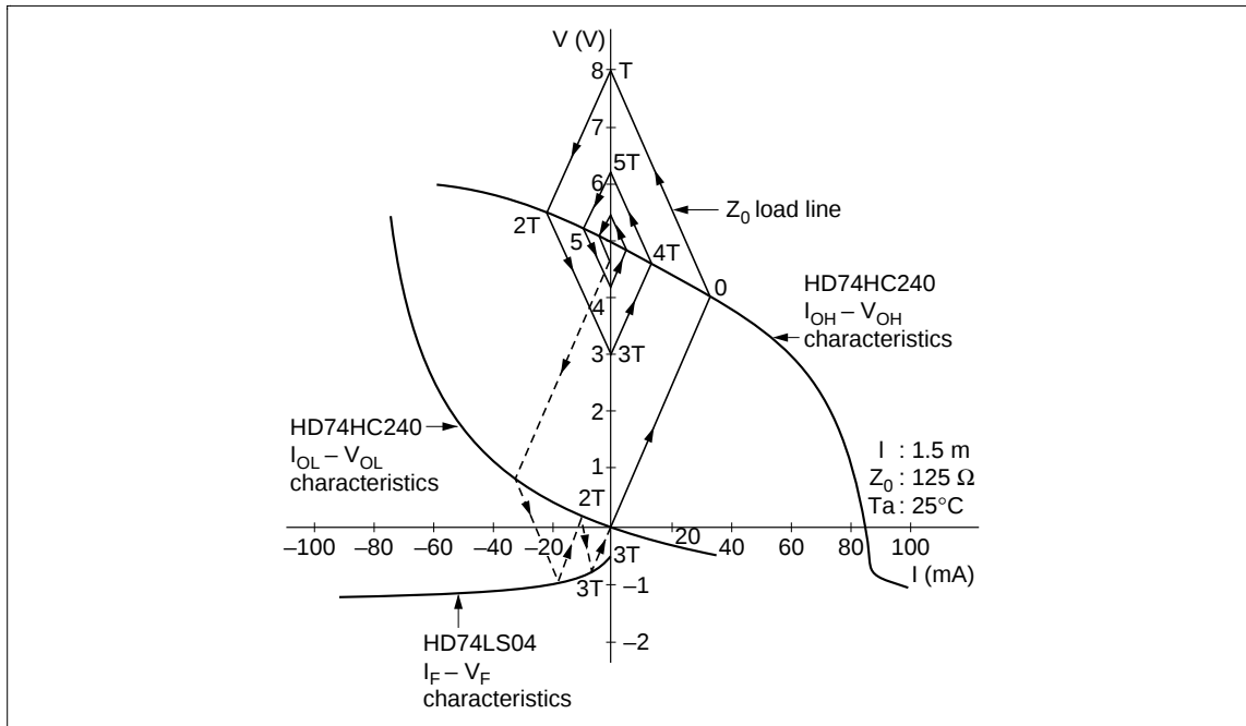
Figure 17 Bergeron Diagram Analysis of the Transmission Model
