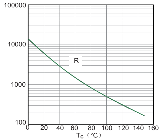
Figure 10: NTC Characteristics
