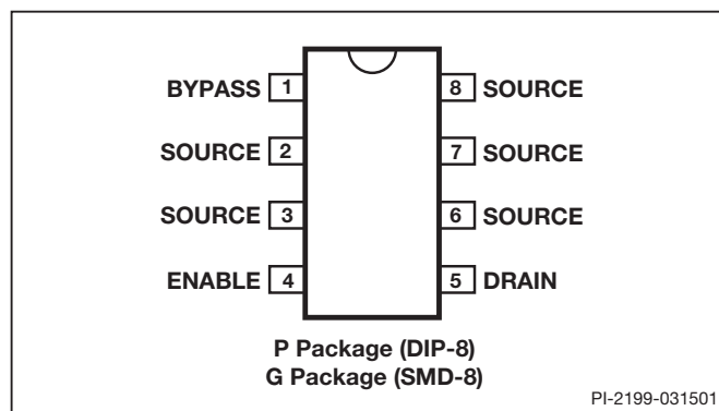
Figure 3. Pin Configuration.
