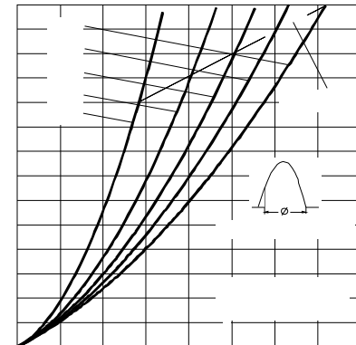
Fig. 5 - On-State Power Loss Characteristics
