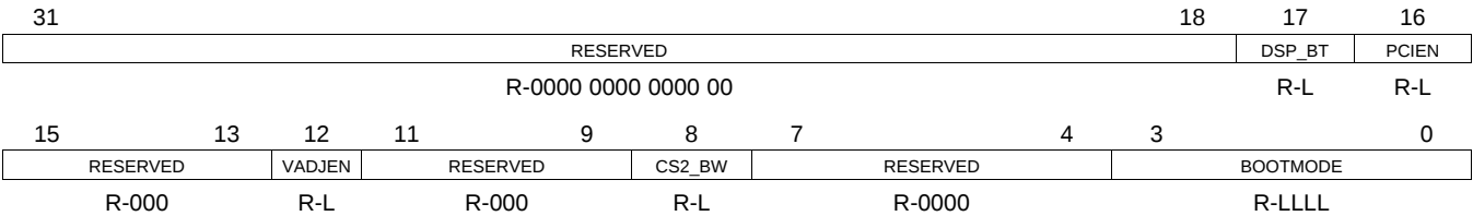
Figure 4-8. BOOTCFG Register
