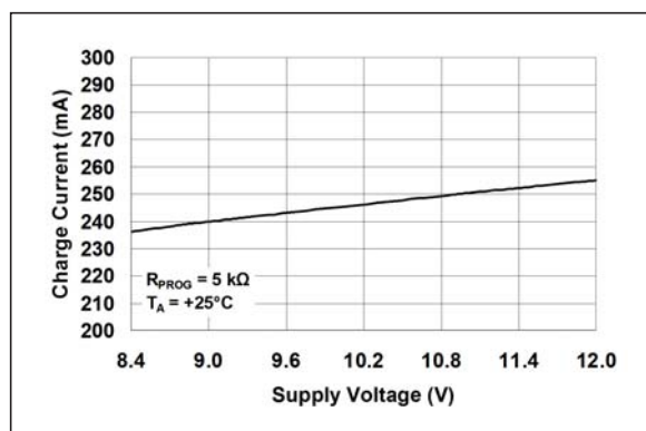
FIGURE 2-8: Charge Current ( I_{OUT} ) vs. Supply Voltage ( V_{DD} ).
