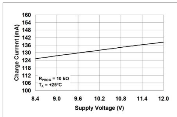
FIGURE 2-7: Charge Current ( I_{OUT} ) vs. Supply Voltage ( V_{DD} ).
