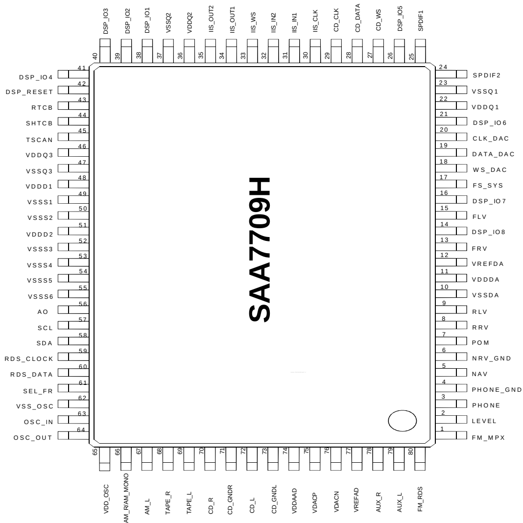
Fig 6.1 Pinning diagram
