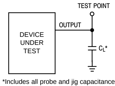
Figure 6. Test Circuit
