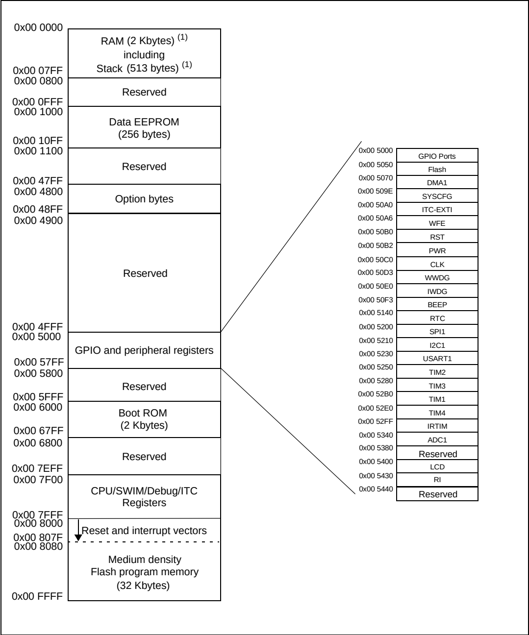
Figure 4. Memory map
