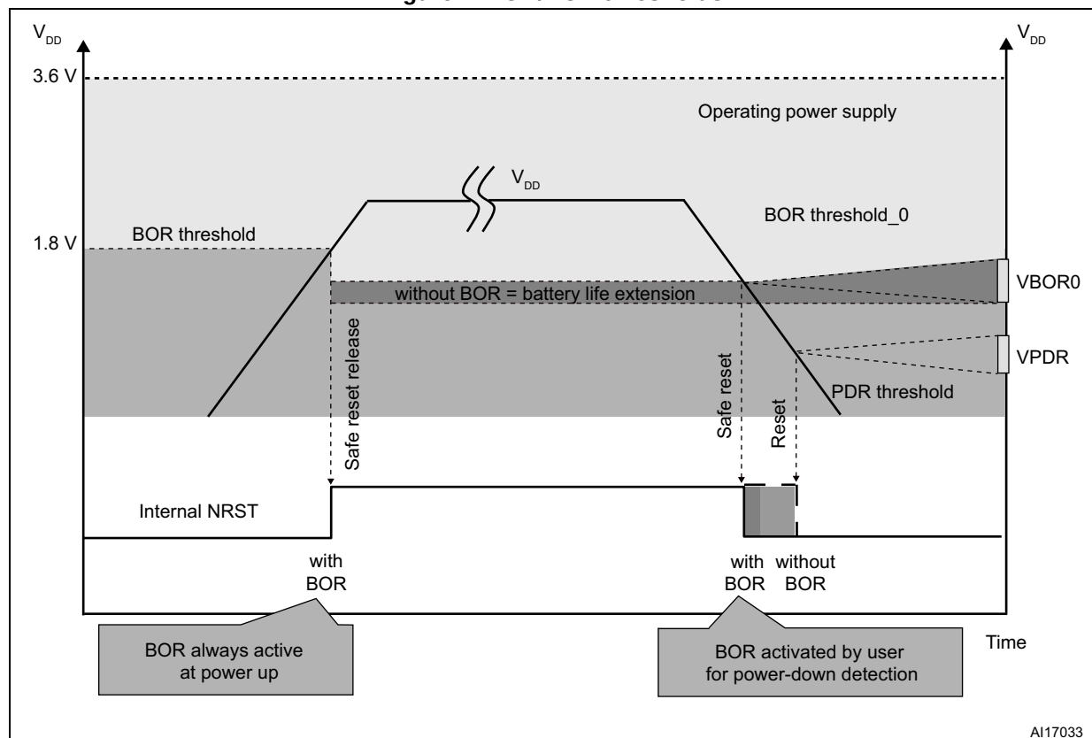
Figure 7. POR/BOR thresholds
