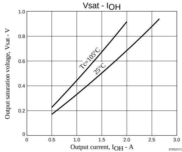
STK672-732B-E Output saturation voltage, V_{sat} - Output current, I_{OH}
