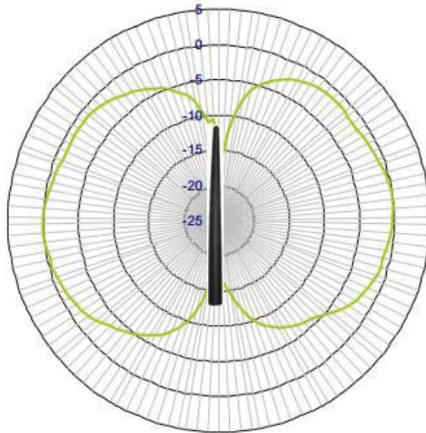
E Field Radiation Pattern
