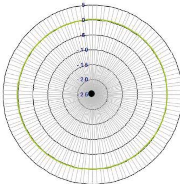
H Field Radiation Pattern
