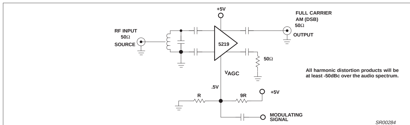
Figure 12. AM Modulator
