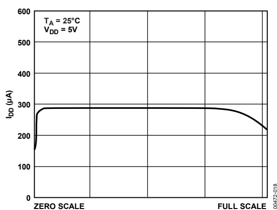
Figure 18. Supply Current vs. Code
