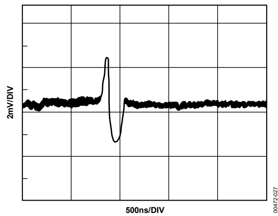
Figure 27. DAC-to-DAC Crosstalk
