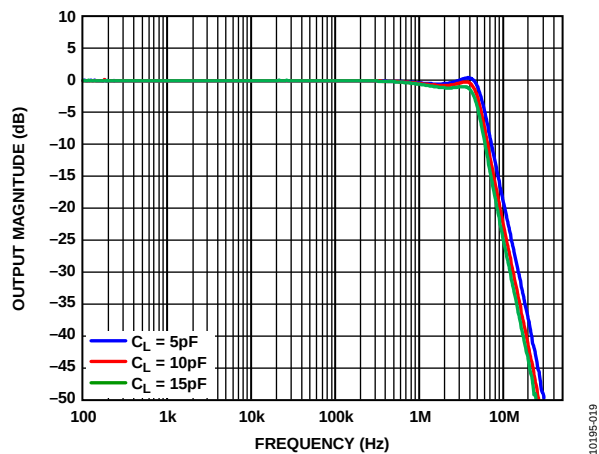
Figure 19. Small Signal Frequency Response for Various Capacitive Loads
