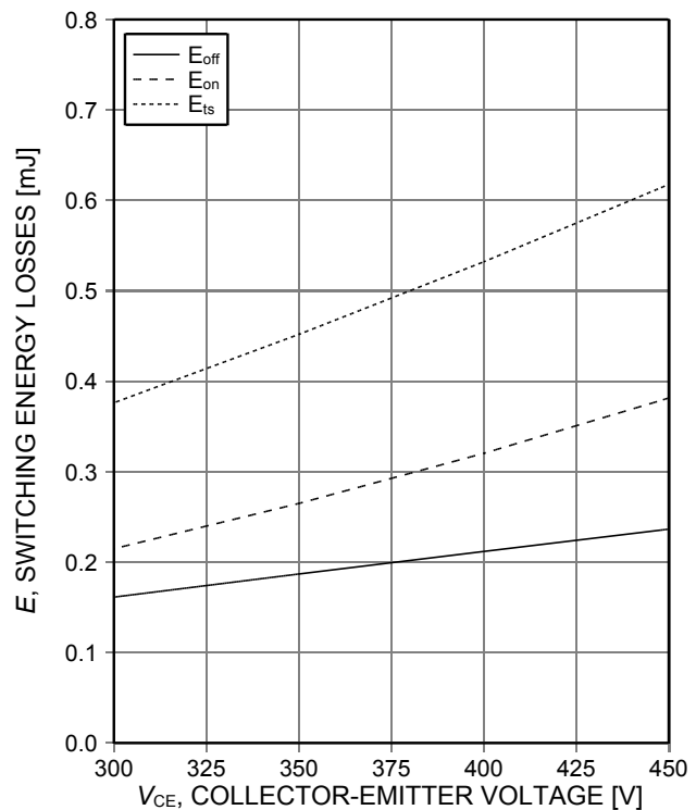
Figure 16. Typical switching energy losses as a function of collector-emitter voltage (inductive load, T_{vj}=175^{\circ}\text{C} , V_{GE}=15/0\text{V} , I_C=10\text{A} , r_G=26\Omega , Dynamic test circuit in Figure E)
