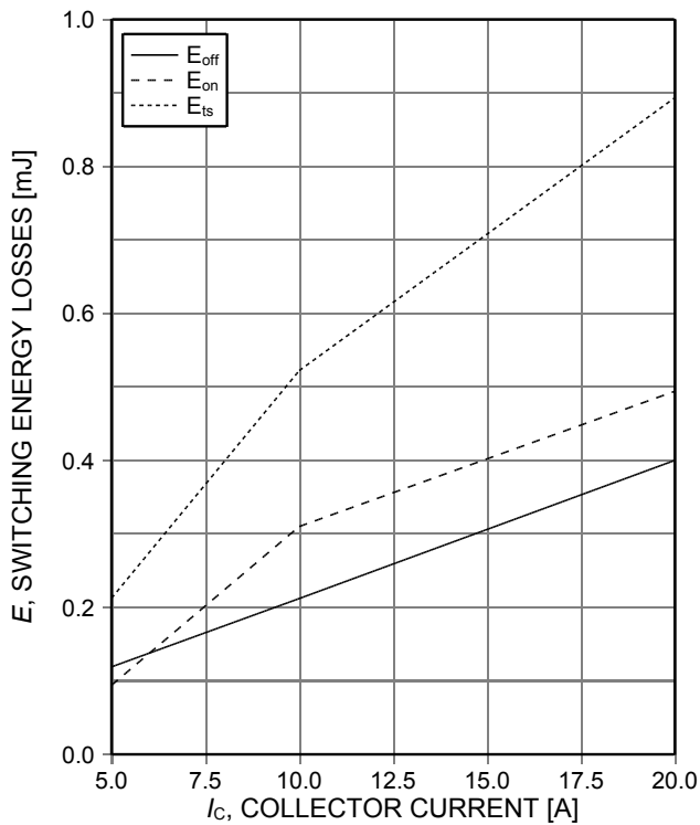
Figure 13. Typical switching energy losses as a function of collector current (inductive load, T_{vj}=175^{\circ}\text{C} , V_{CE}=400\text{V} , V_{GE}=15/0\text{V} , r_G=26\Omega , Dynamic test circuit in Figure E)
