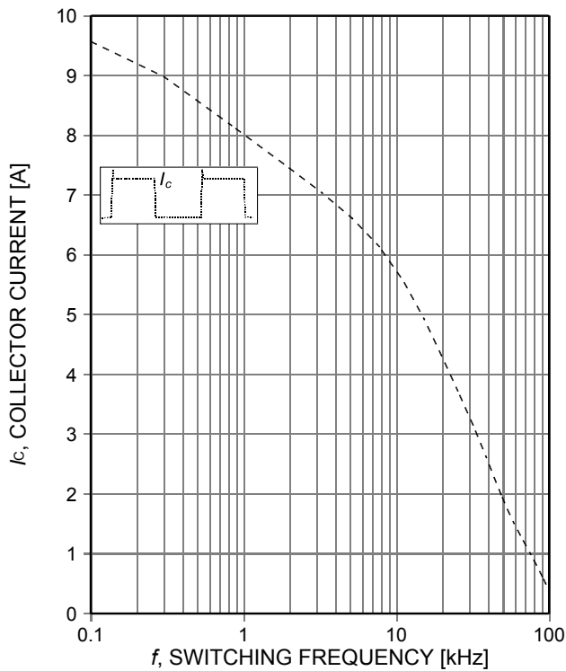
Figure 1. Collector current as a function of switching frequency (T_{vj} \leq 175^\circ\text{C}, T_a = 55^\circ\text{C}, D = 0.5, V_{CE} = 400\text{V}, V_{GE} = 15/0\text{V}, r_G = 26\Omega, \text{PCB mounting with thermal vias and heatsink, see Appnote: } \text{www.infineon.com/igbt})
