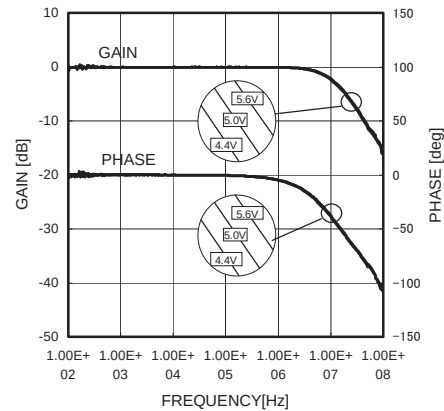
Fig5. Frequency characteristics (Supply voltage dependence)
