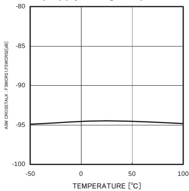
Fig12. MUTE Attenuation
