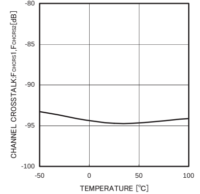
Fig14. Channel Crosstalk
