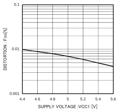
Fig7. Distortion (Supply voltage dependence)
