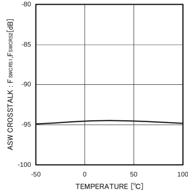
Fig13. ASW Crosstalk
