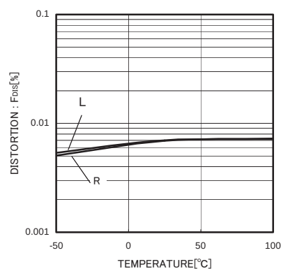
Fig8. Distortion (Temperature dependence)
