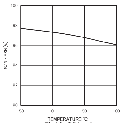
Fig10. S/N ratio (Temperature dependence)
