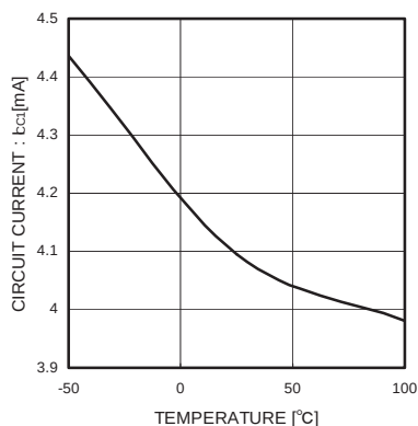
Fig3. Circuit Current1
