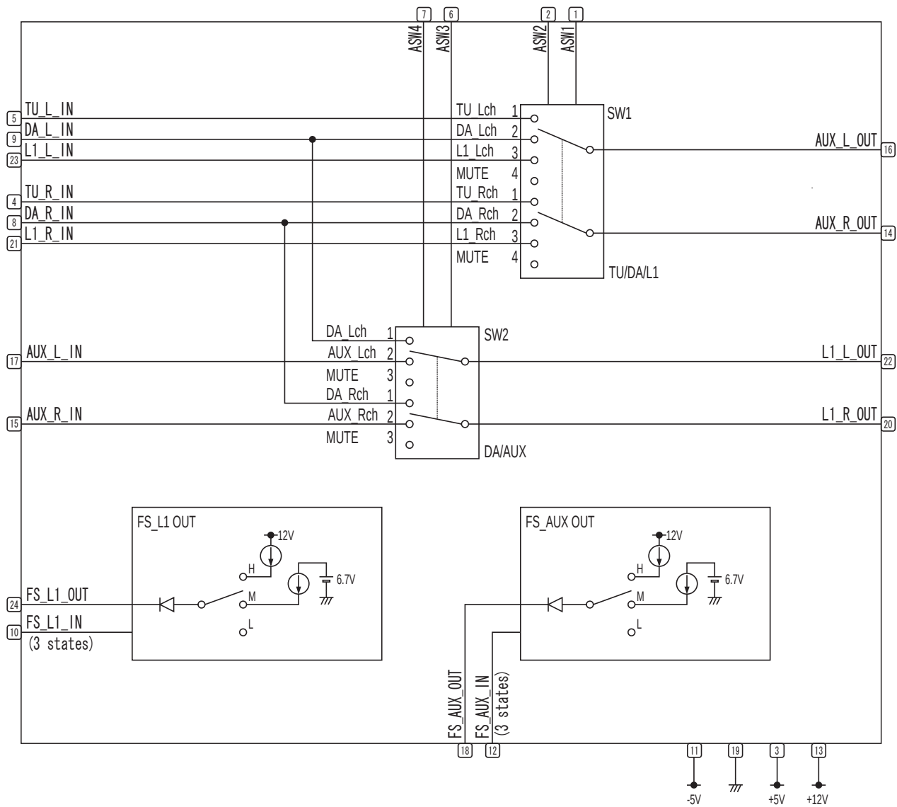
Fig.1 Block Diagram
