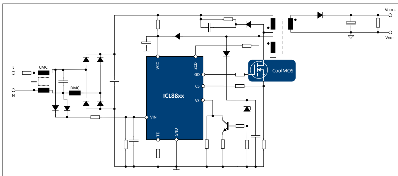
Figure 2 Flyback-PSR-CV
