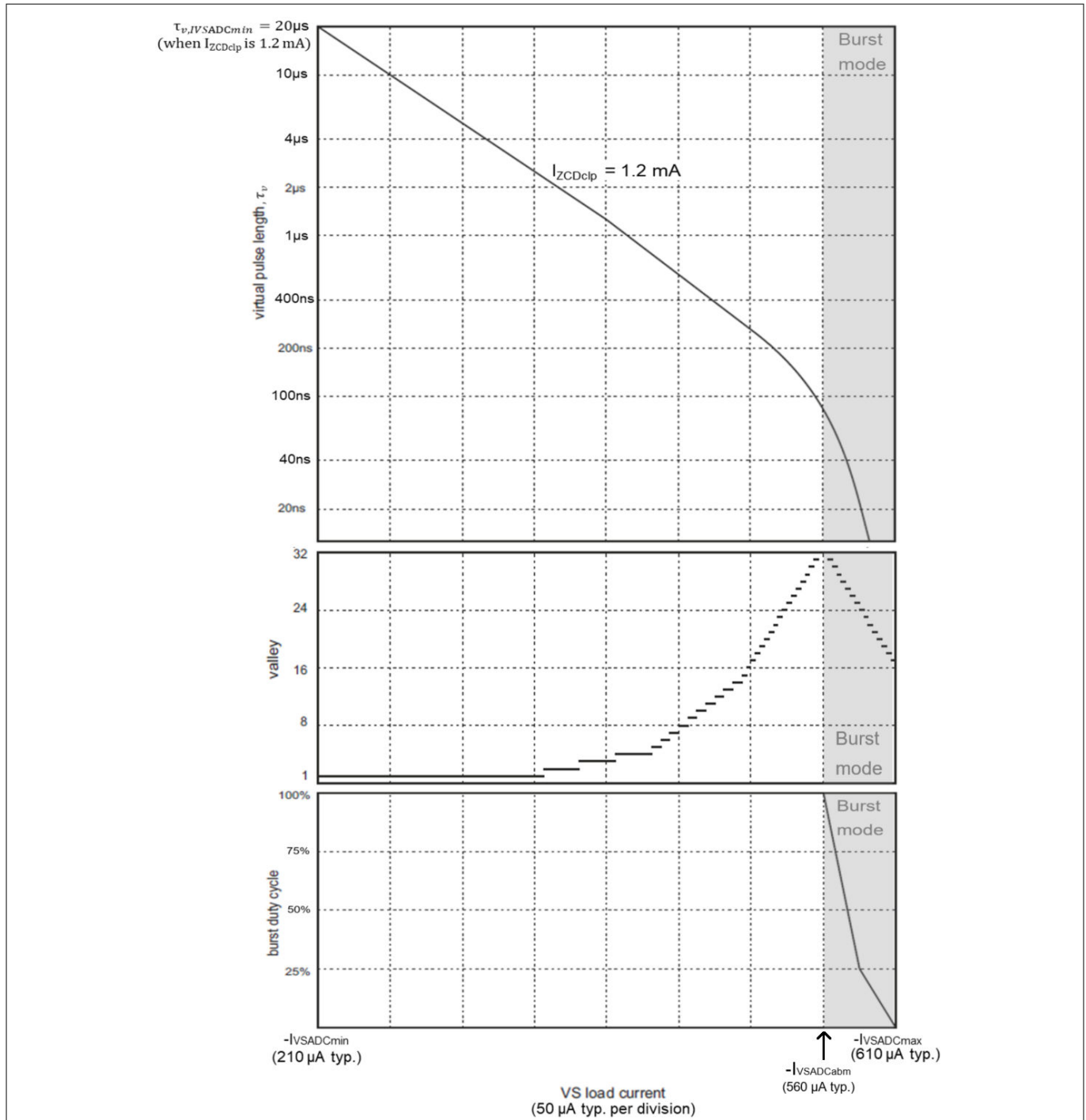
Figure 12 Virtual pulse length mapping (based on I_{ZCDclp} = 1.2 mA as an example), valley number mapping and burst mode mapping (burst mode applies to ICL8810 and ICL8820 only)
